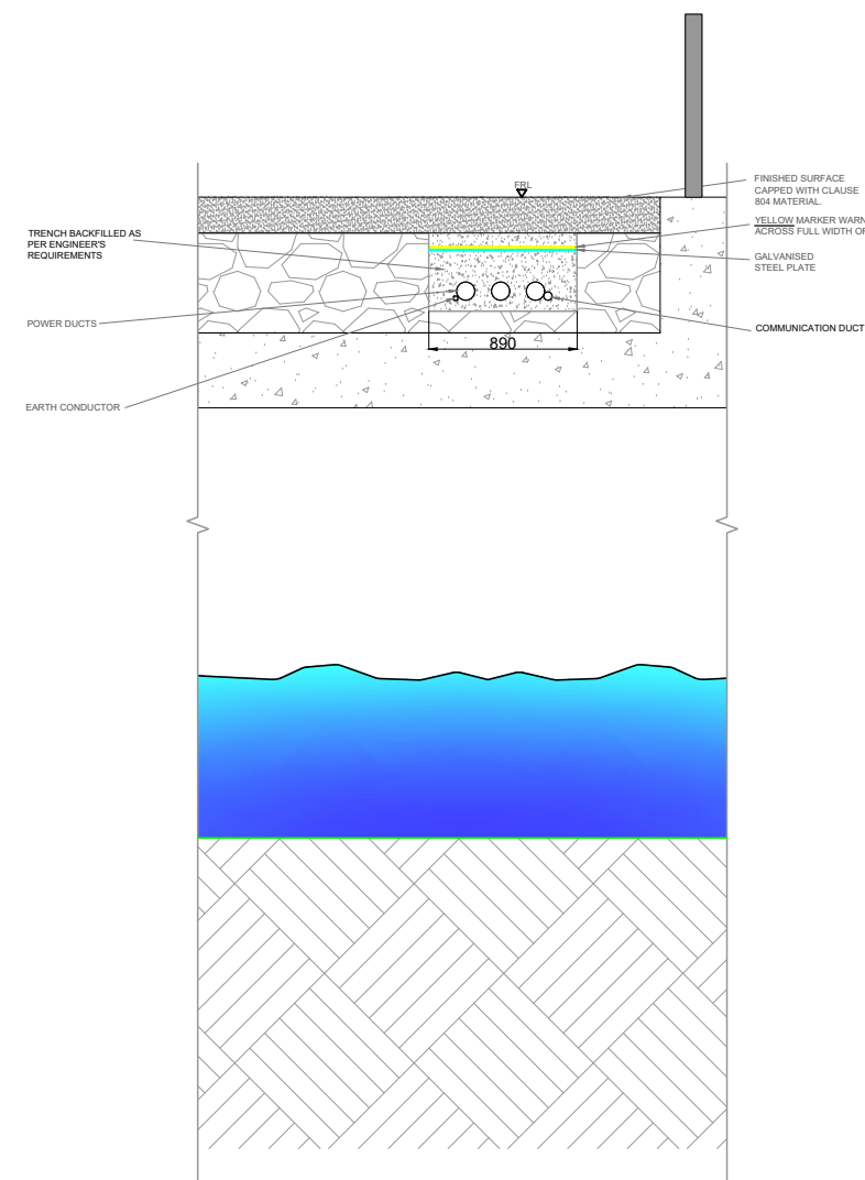
Clear Span Watercourse Crossing - 33kV - Cross Section
