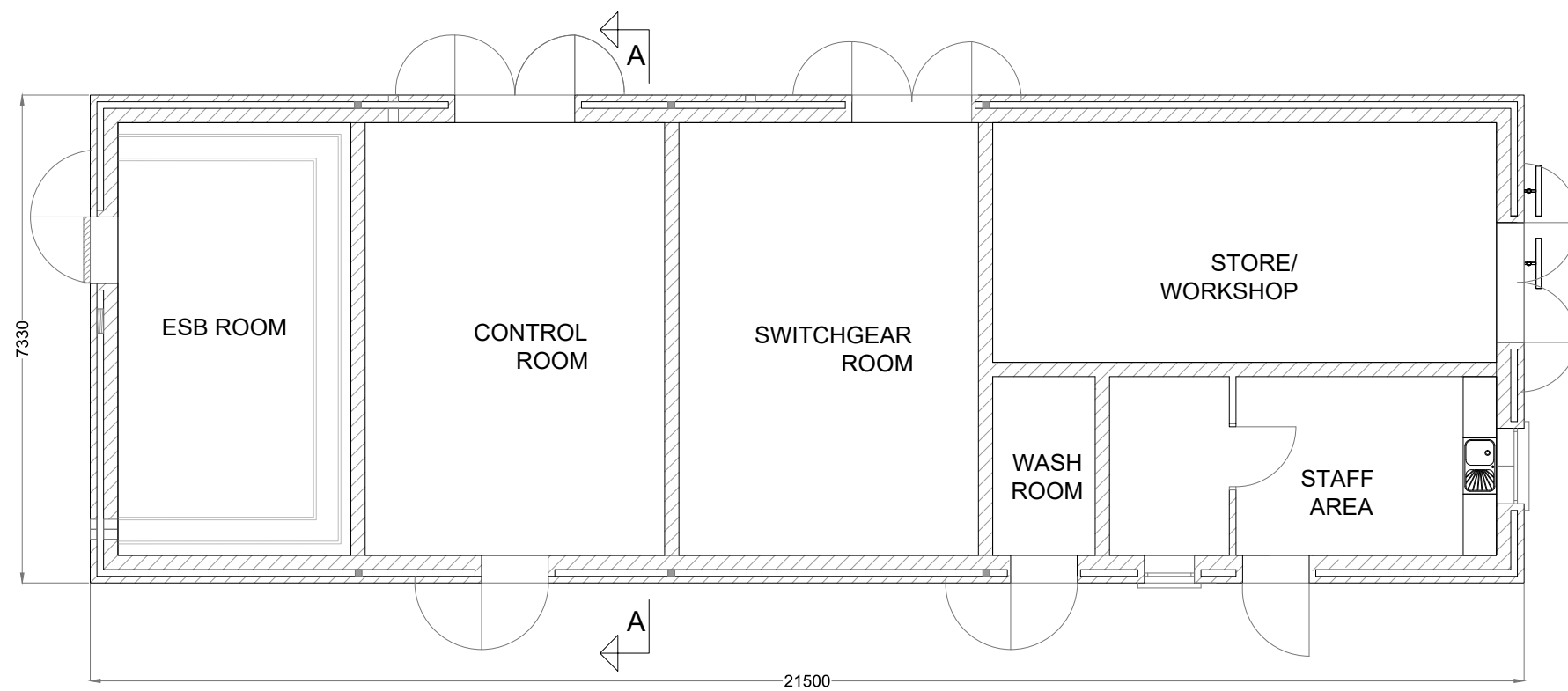
Proposed 38 kV Control Building Layout Plan 1:100
