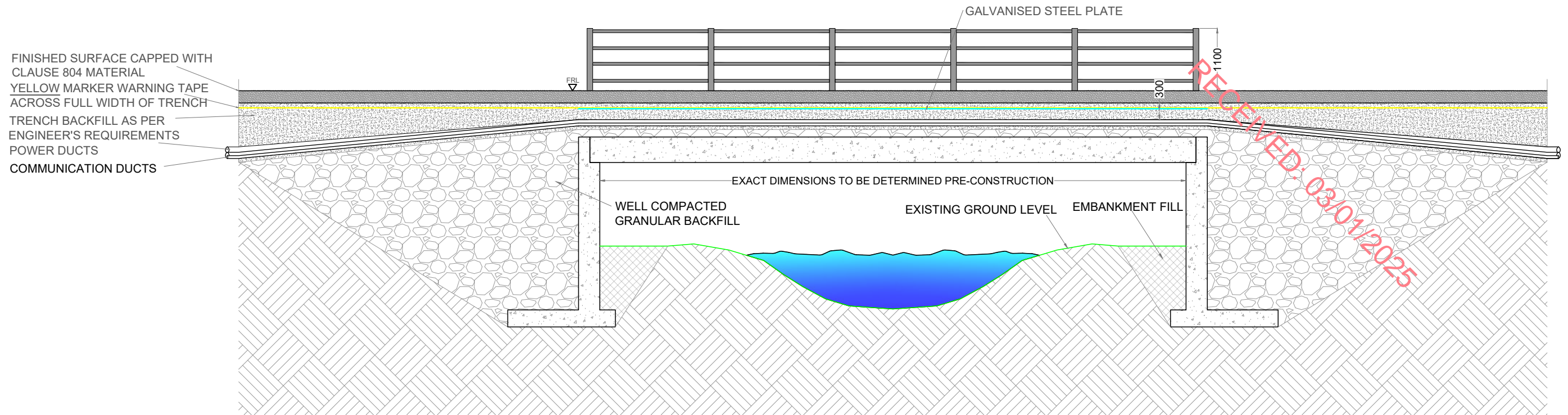
Clear Span Watercourse Crossing - 33kV - Longitudinal Section
